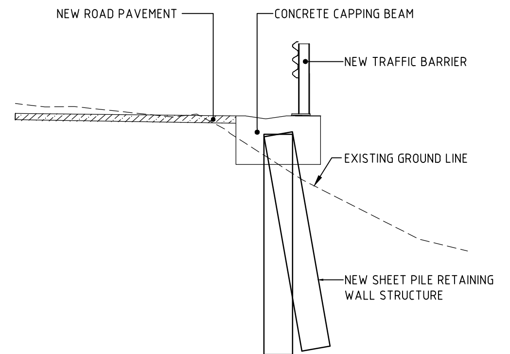
TYPICAL SHEET PILE RETAINING WALL SECTION
