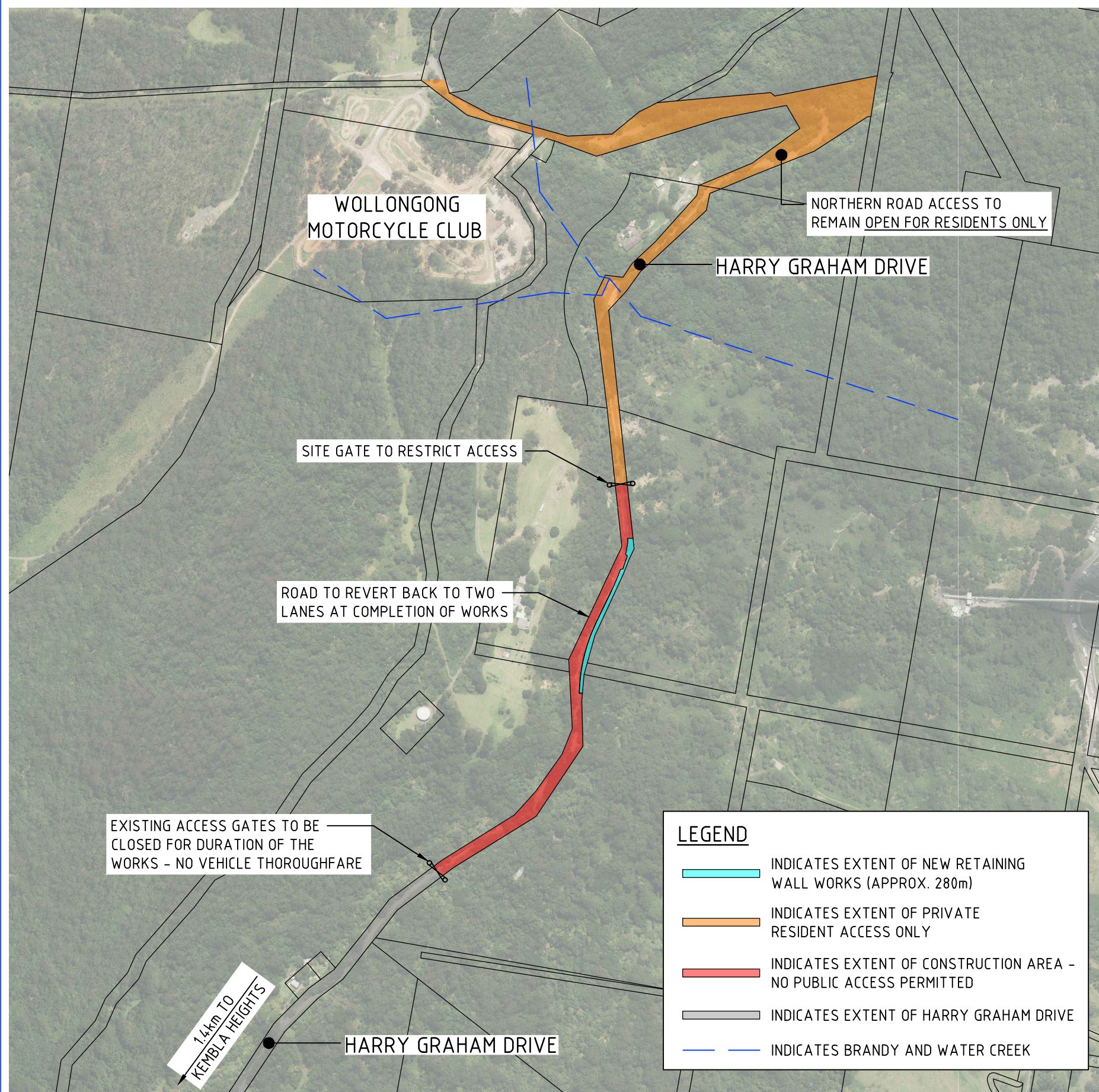
PROPOSED WORKS AREA PLAN
